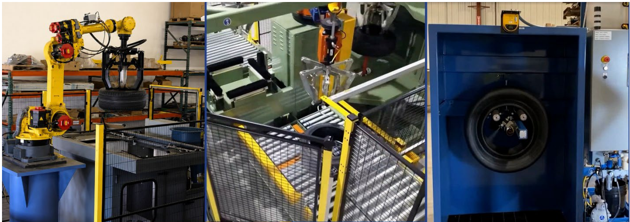
Green Tire Spraying Systems
